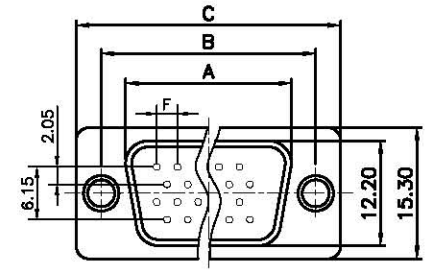
78pin Figure
